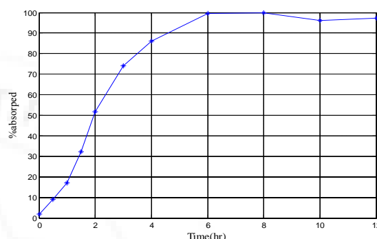
Figure 2: Percent Absorbed Versus time using Wagner-Nelson Method
