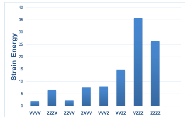
Figure 6 Strain energy at the failure point of each specimen.
