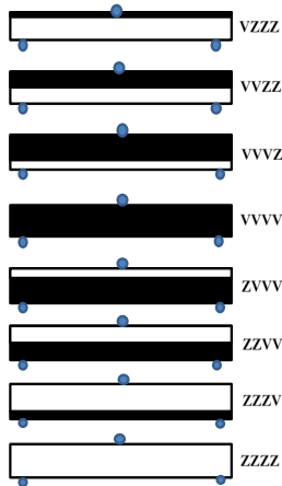
Figure 1 The eight specimens with different configurations.
