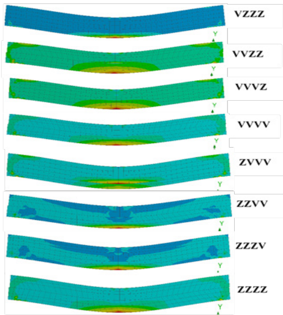
Figure 4 Maximal principal stresses distribution in all specimens.
