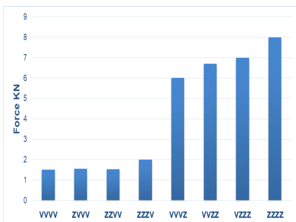
Figure 5 Failure force of each specimen.
