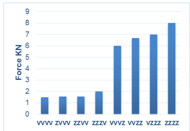
Figure 3 Fracture loads.
